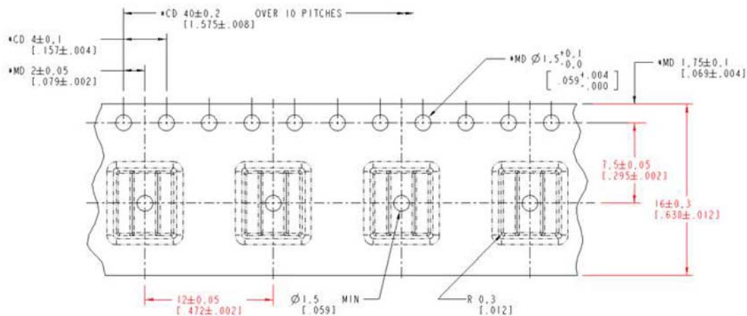
Figure 2: 70ABJ-4-Male Improved Design
